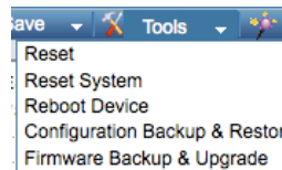
Figure 38 – Tool Menu
