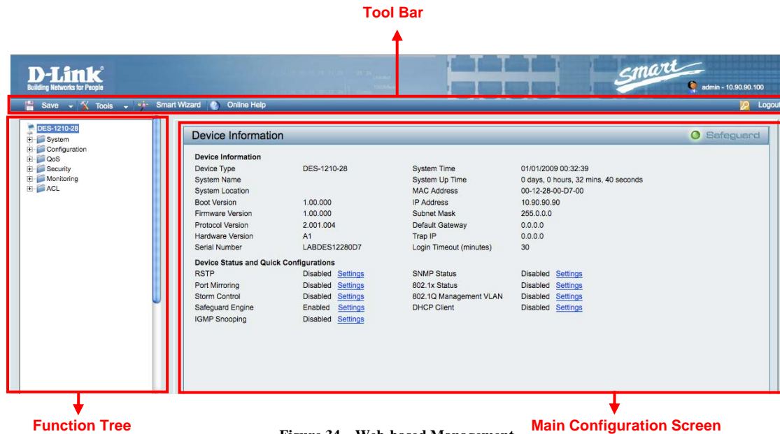
Figure 34 – Web-based Management
