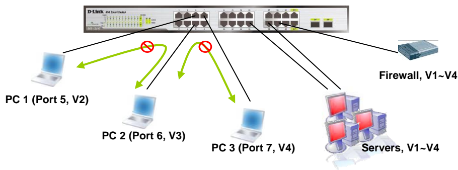
Figure 66 – Configuration > 802.1Q VLAN > Asymmetric VLAN Example
