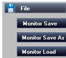
Figure 21 – SmartConsole File
