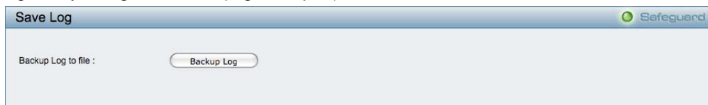
Figure 37 – Save Log
