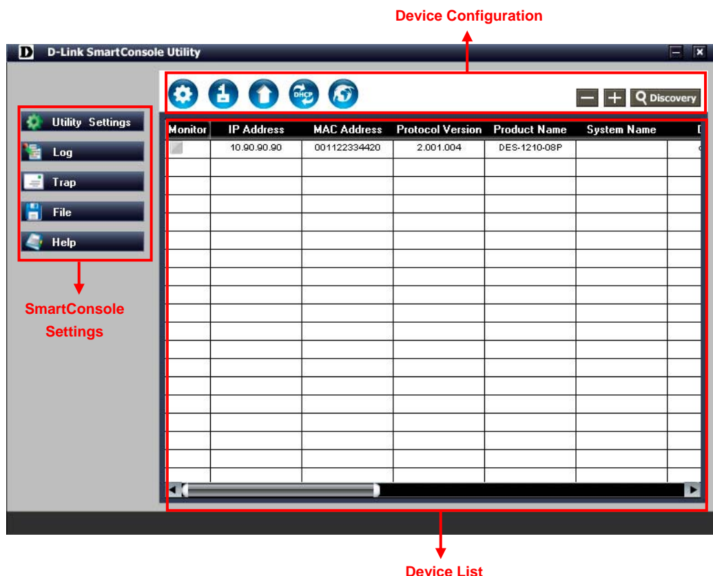
Figure 17 – SmartConsole Utility
