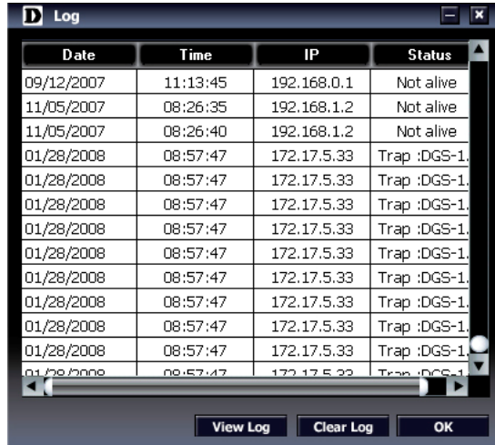
Figure 19 – SmartConsole Log
