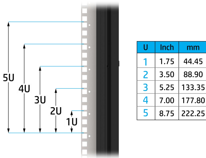
Fig 5 – Layout and dimensions of a 5U rack space
