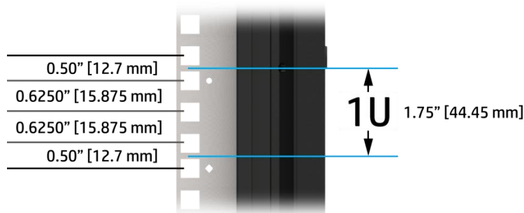
Fig 6 – Rack mounting hole positioning in 1U rack space
