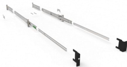
Fig 4 – The HP Z6/Z8 Rack Mount kit (B8S55AA) components
